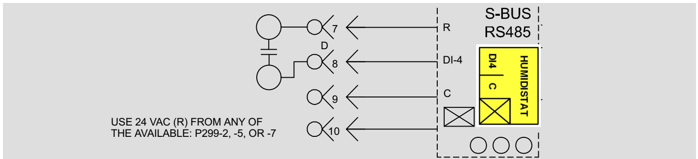
Figure 7. Humiditrol Reheat Diagram (ECTO 4.25 set to 100 for digital control)
