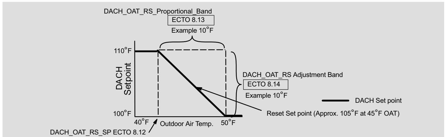
Figure 24. Outdoor Air Reset Example
